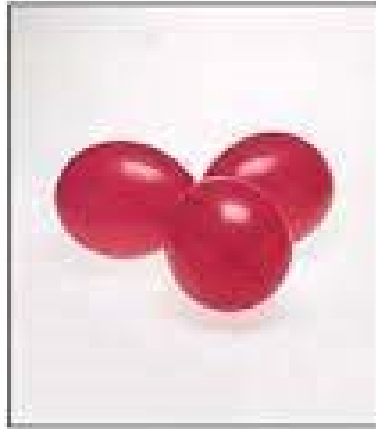
Trigonal planar
